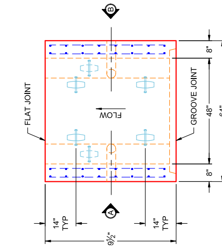
PLAN VIEW PC 1 (UPRIGHT IN MOLD)
