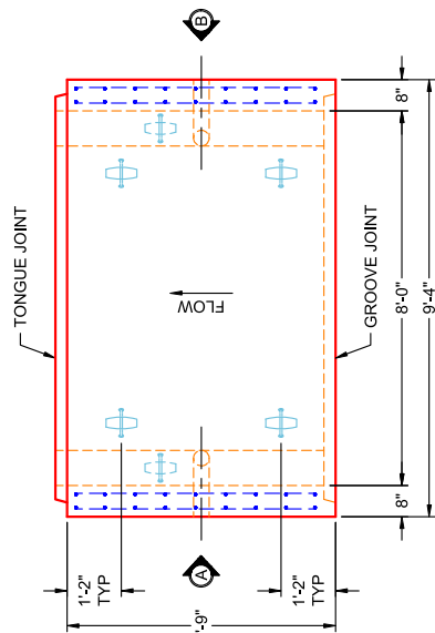
PLAN VIEW PC 8
