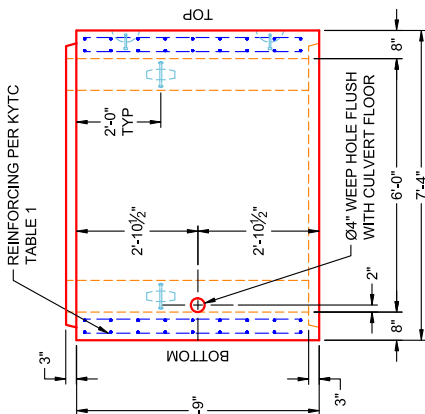
VIEW A PC 8
