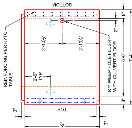
VIEW B PC 23
