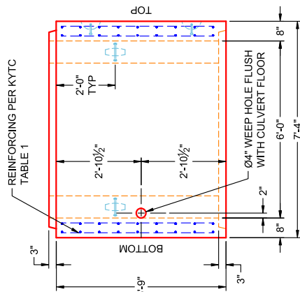
VIEW A PC 23
