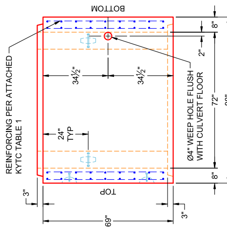
VIEW B PC 23 (UPRIGHT IN MOLD)
