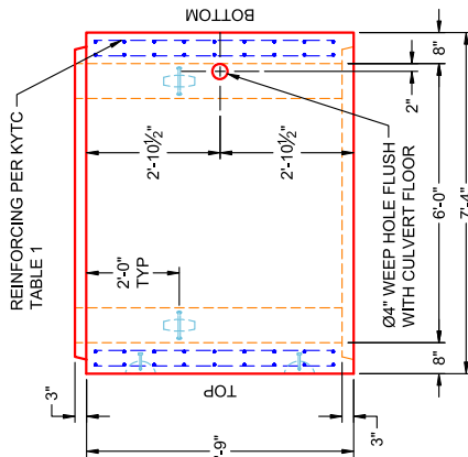
VIEW B PC 22
