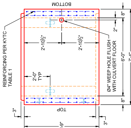
VIEW B PC 21
