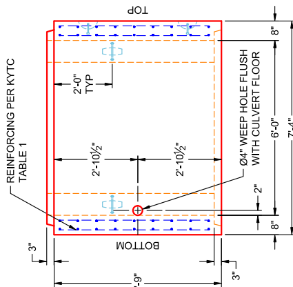
VIEW A PC 21
