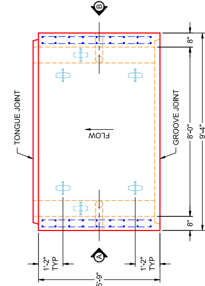
PLAN VIEW PC 17
