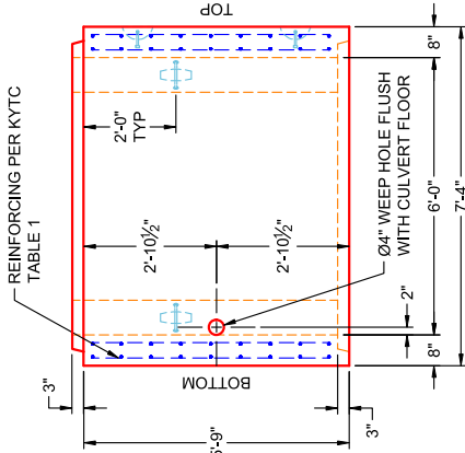
VIEW A PC 12
