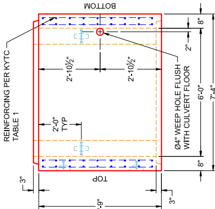
VIEW B PC 12
