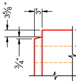
JOINT DETAIL (TYP) NTS
