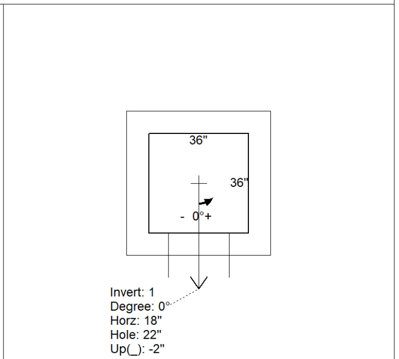
UPSIDE-DOWN VIEW (int. dimenions)
