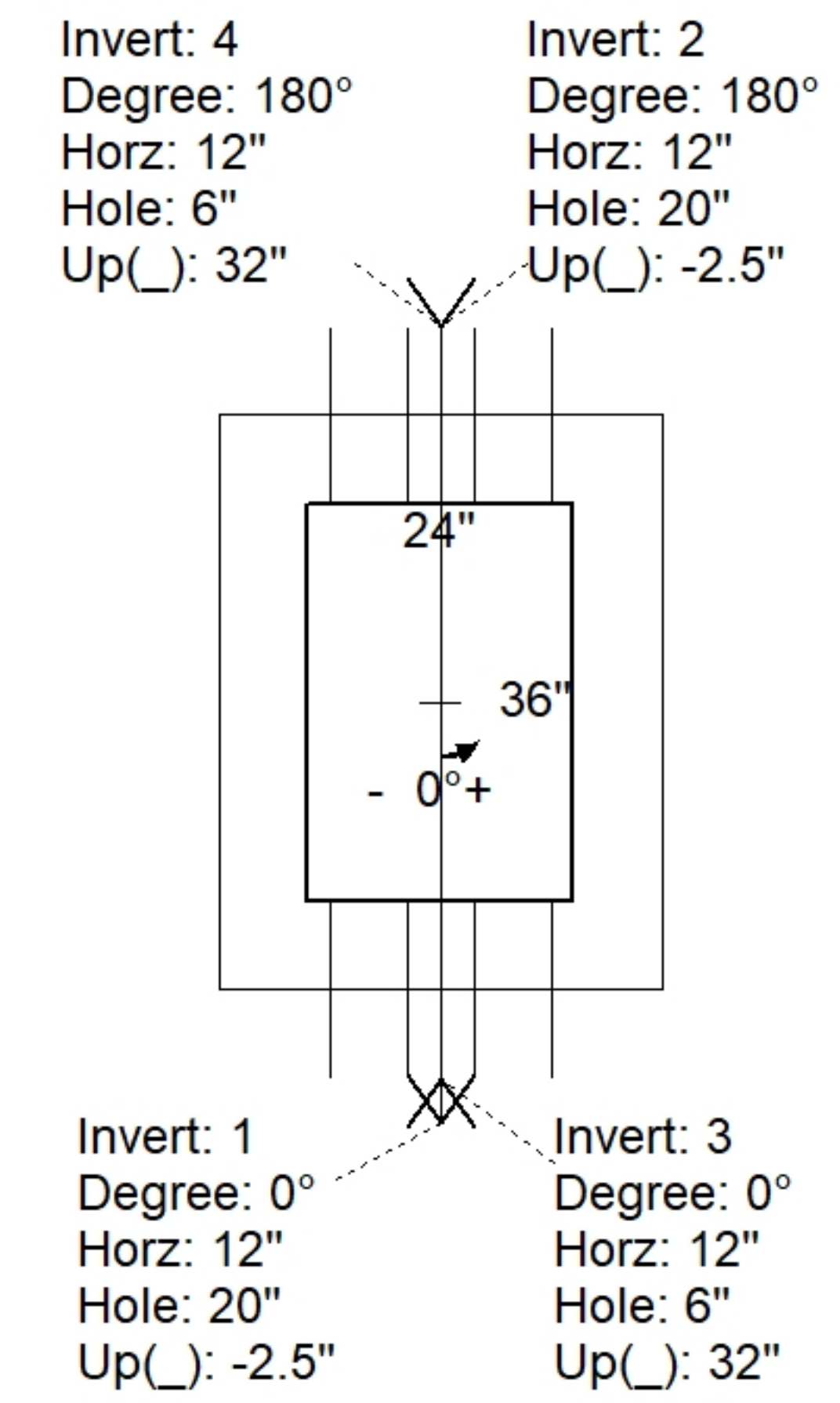
UPSIDE-DOWN VIEW (int. dimensions)
