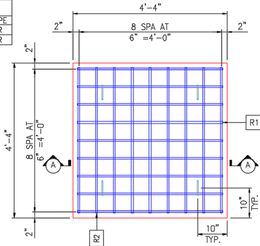
PLAN VIEW
