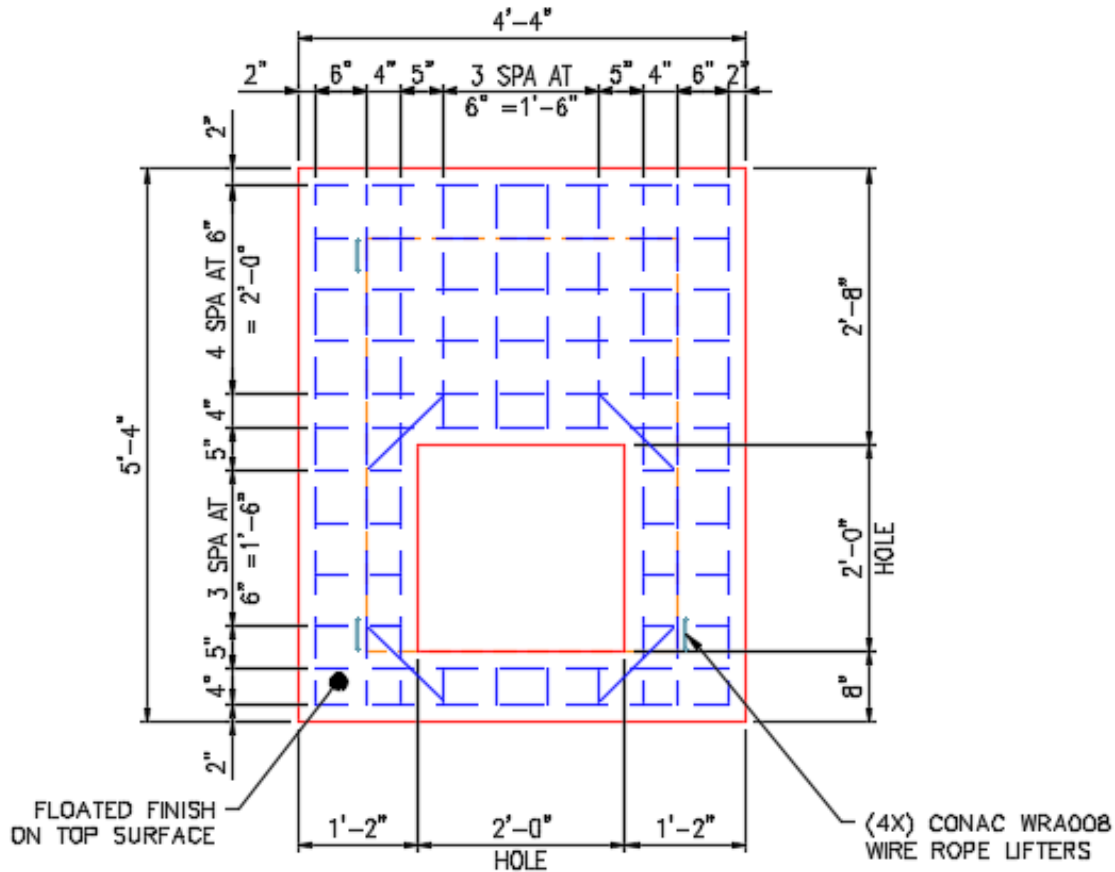
PLAN VIEW
