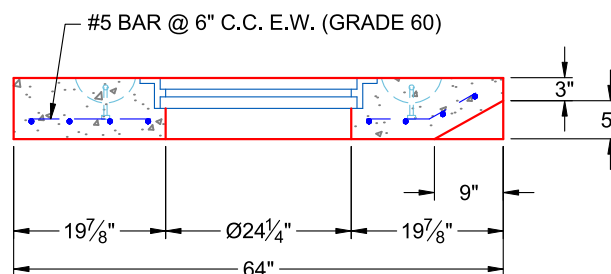
SECTION B-B (RIGHT SIDE UP)
