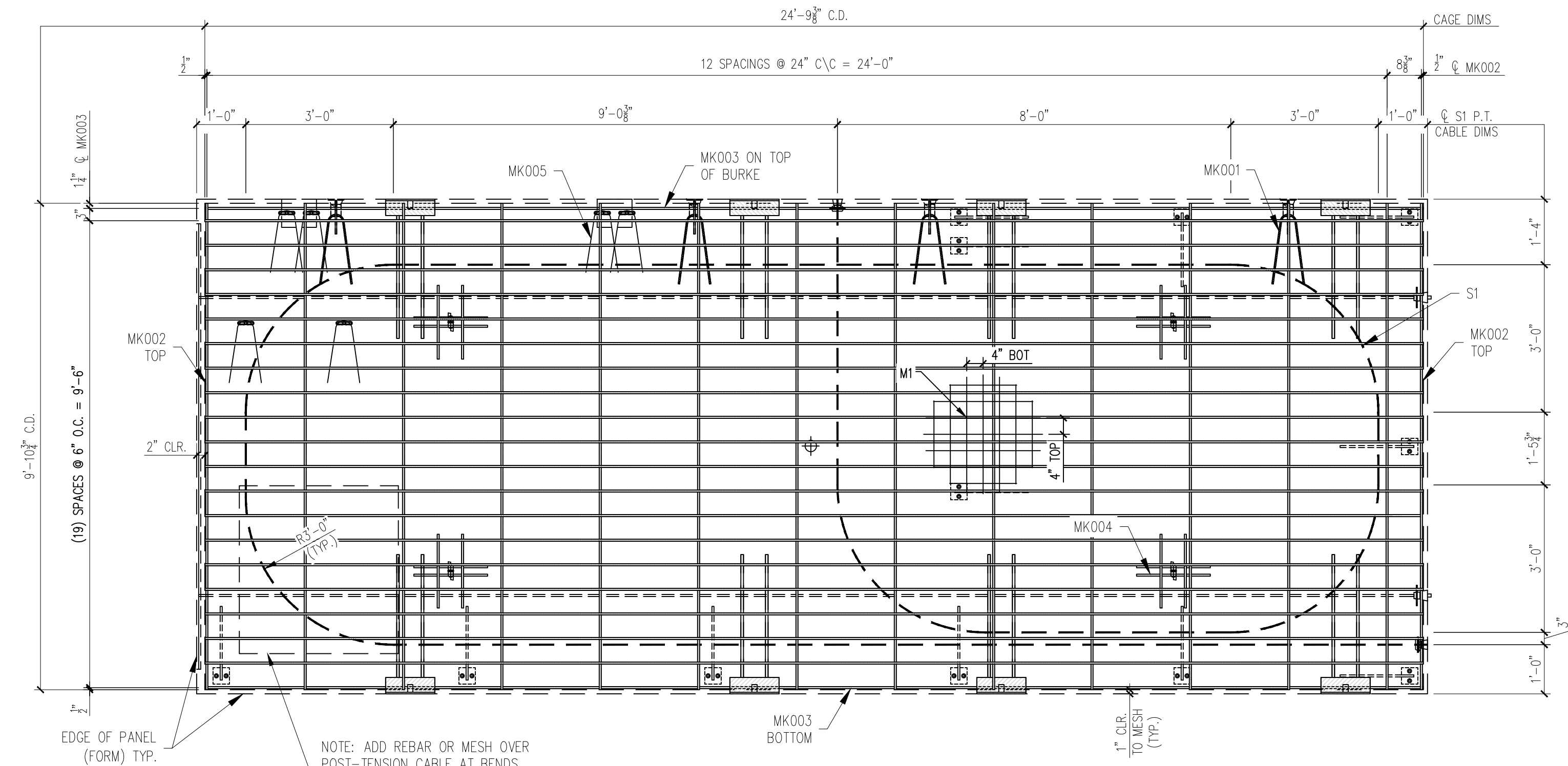
FLOOR REINFORCING VIEW SCALE: \frac{1}{2} " = 1'-0"
